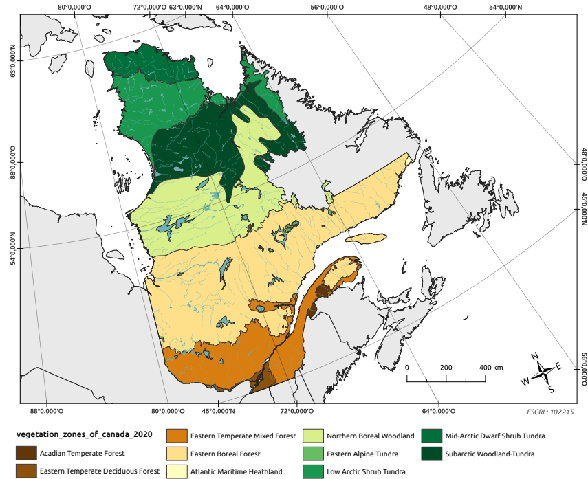
Figure 10: Vegetation Zones of Canada in 2020 from [9]. This map highlights three different regions: the Temperature region in the south, the Boreal region in the centre of the country, and the Arctic region in the north of Quebec.
