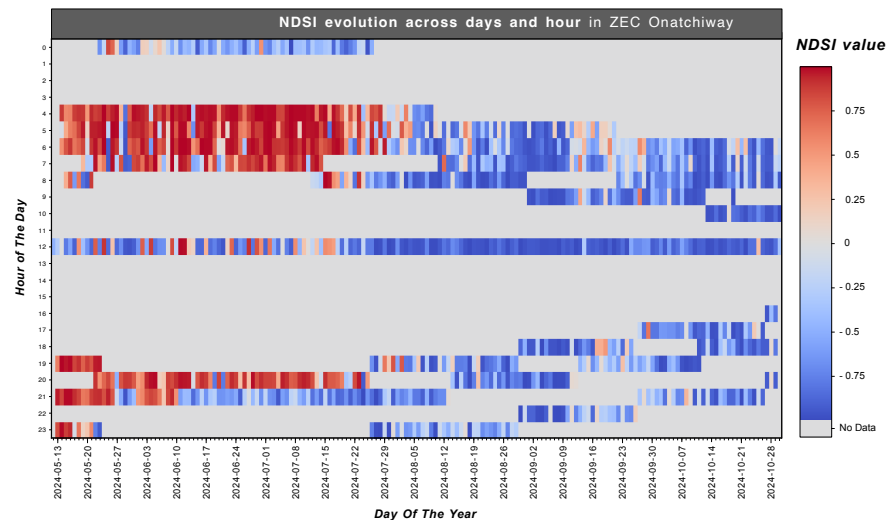
Figure 85: Evolution of the NDSI value across days and hours in the ZEC Onatchiway station
