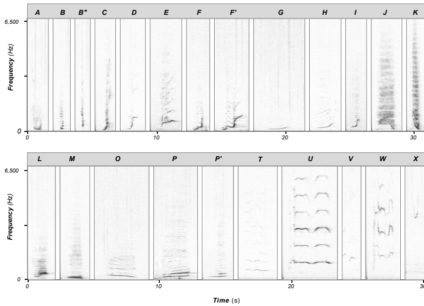
Figure 15: Spectrogram for each unit of the North Atlantic humpback whale's vocal repertoire on breeding grounds. The global spectrogram was generated using a Short-Term Fourier Transform (STFT), signals resampled at 13 kHz, 2048-point Hanning window and 1400-point overlap
