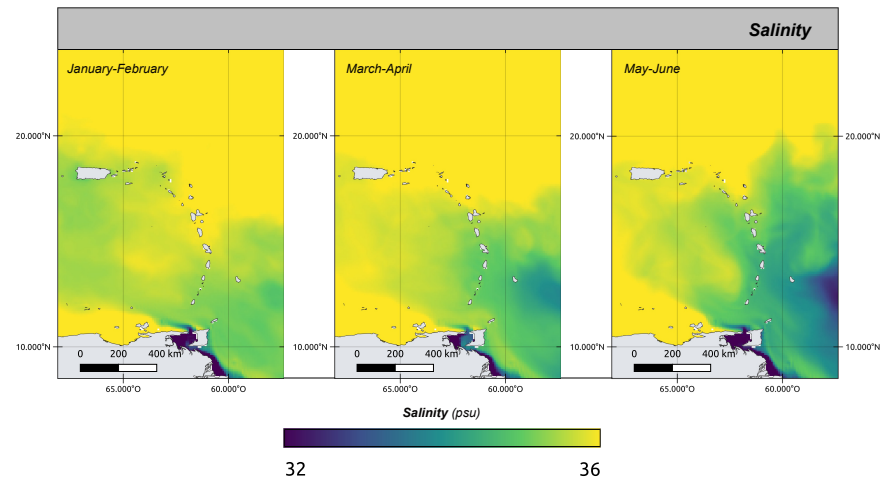
Figure 58: Surface salinity evolution over 3 periods of time in the Caribbean.
