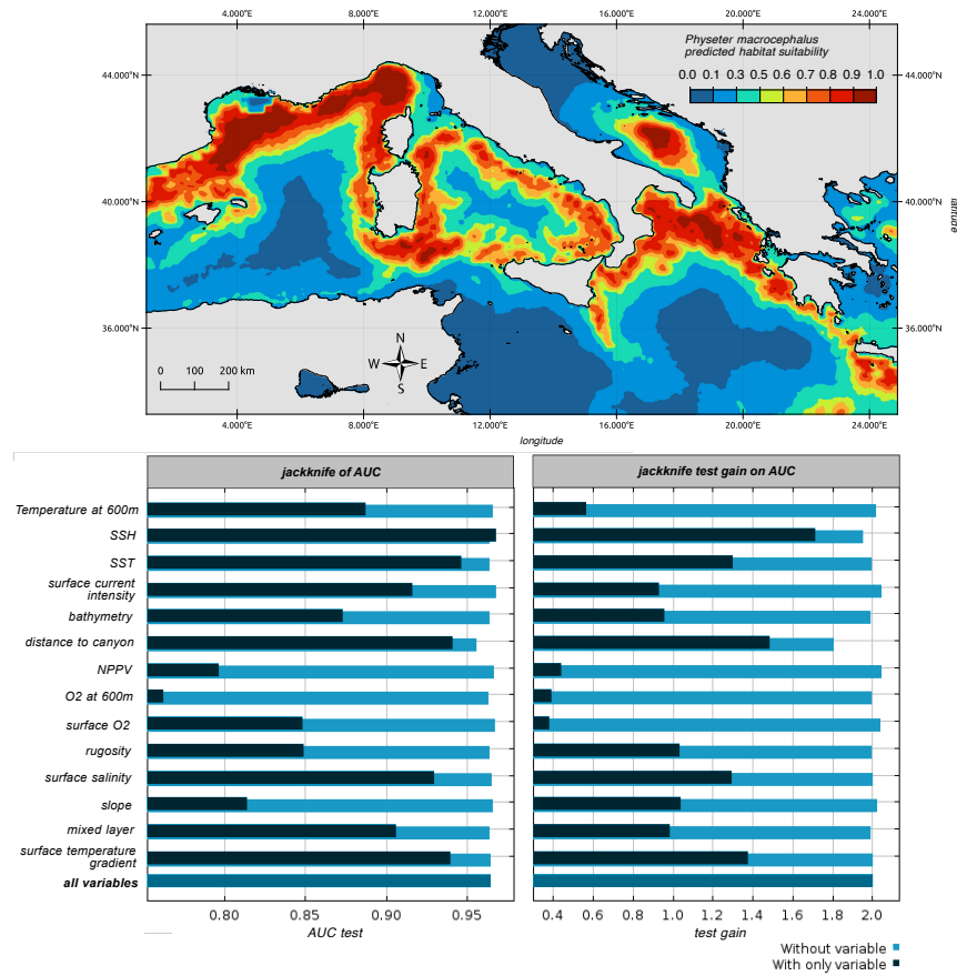
Figure 64: Result of the MaxENT model using all fixed and variable parameters.
