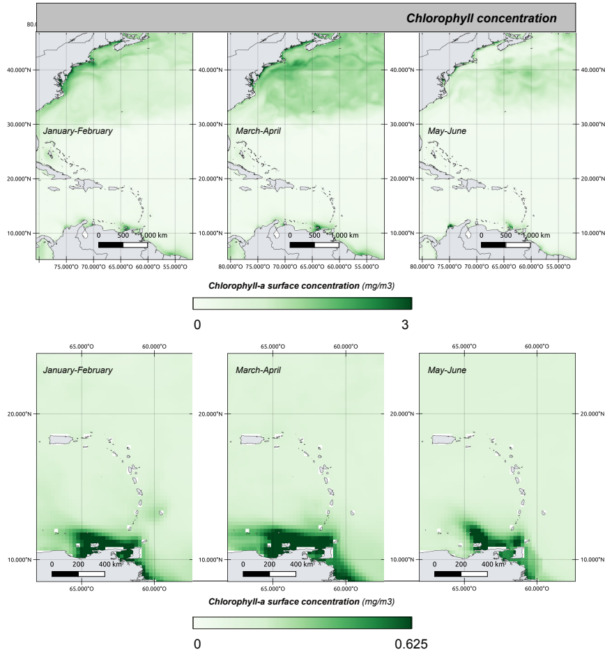
Figure 57: Chlorophyll-a concentration over 3 periods of time in the Northern Atlantic (top) and the Caribbean (bottom).
