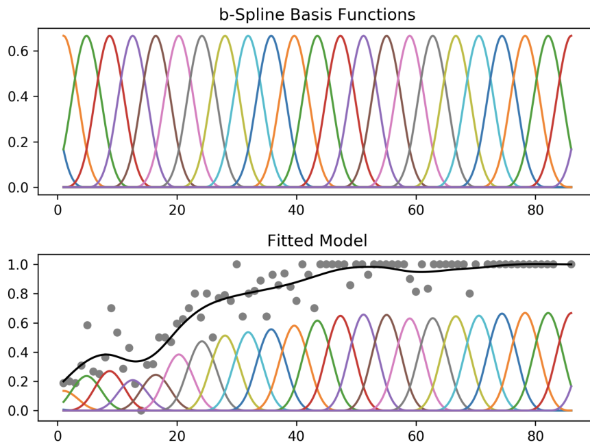
Figure 21: Representation of the splines that make up the Generalized Additive Model (GAM) (top), and the fitted model representation (bottom).
