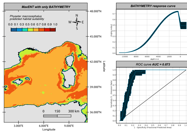
Figure 46: MaxENT model projection using the bathymetry, with the response curve and its ROC AUC over the test set OBIS.
