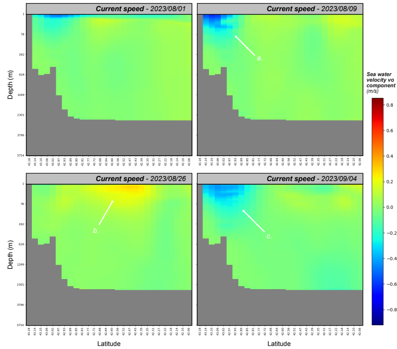
Figure 80: Current northward component evolution during different days for a depth latitudinal cut. a. the current is from the coast to the sea, which can create downwelling in the area; there is a strong current from the sea to the coast; c : once again a strong current from the coast to the sea, even in deep water of the canyon.
