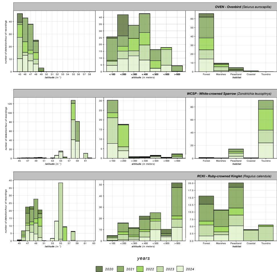
Figure 43: Preferences for latitude, altitude and habitat of the three sample species (OVEN, WCSP and RCKI) between 2020 and 2024.
