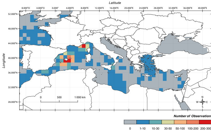
Figure 8: OBIS dataset observation densities across the Mediterranean Sea. The map highlights the two main areas where observations are concentrated: the Ligurian and Balearic regions.
