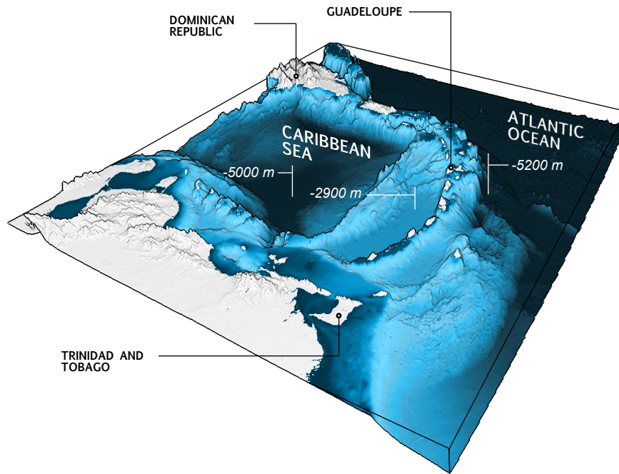
Figure 51: Three-dimensional representation of the Caribbean region incorporating bathymetric information.
