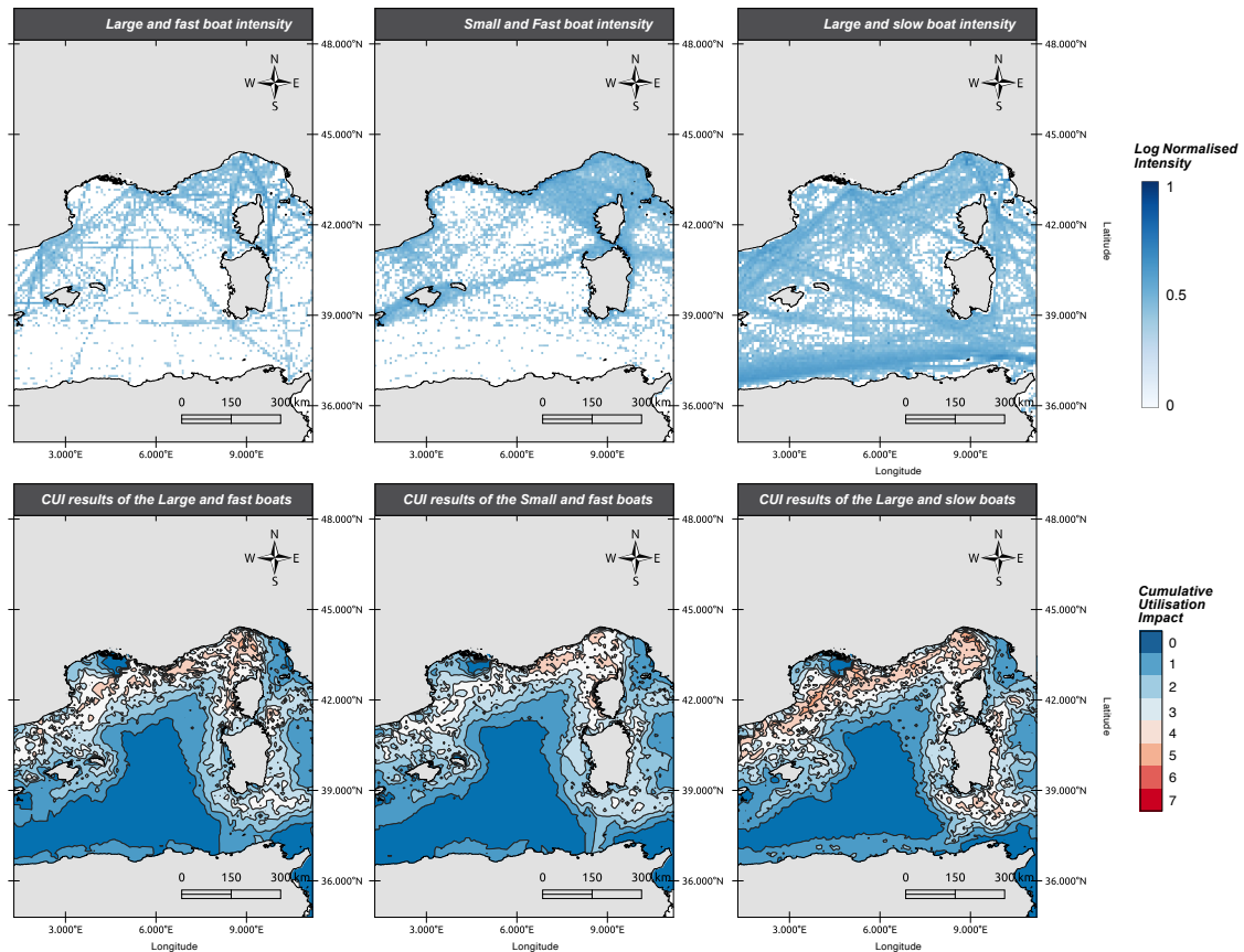
Figure 67: Result of the Cumulative Utilisation Impact (CUI) for each boat categories.
