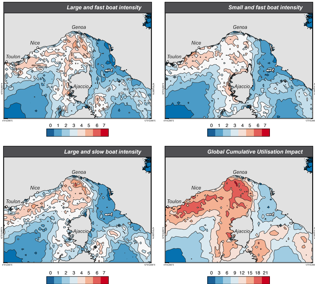
Figure 69: Zoom on the Pelagos Sanctuary for the different boat categories Cumulative Utilisation Impact.
