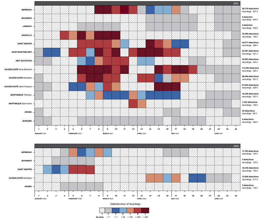
Figure 36: Weekly mean detection per recording hour during the breeding season and over the 14 considered stations. 2021 is represented at the top while 2022 at the bottom. Over the thousands of hours of recordings from the first 6 months, a total of 659,222 detections were kept. A threshold was set to 7 detections per hour of recording to define a week as positive or not. Given that one week represents approximately 27 hours of recording, this represents at least 190 detections, or several dozen minute-long files containing at least 3 detections. The maximum average detection rate is 1,180 per recorded hour.
