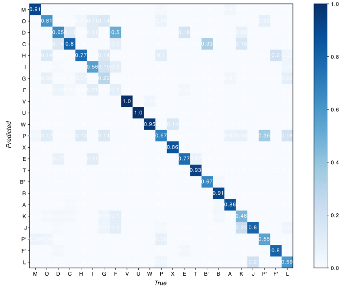
Figure 17: Random Forest confusion matrix over the 23 units of the humpback whale vocal repertoire. The y-axis corresponds to the model's predictions, while the x-axis corresponds to the annotations.
