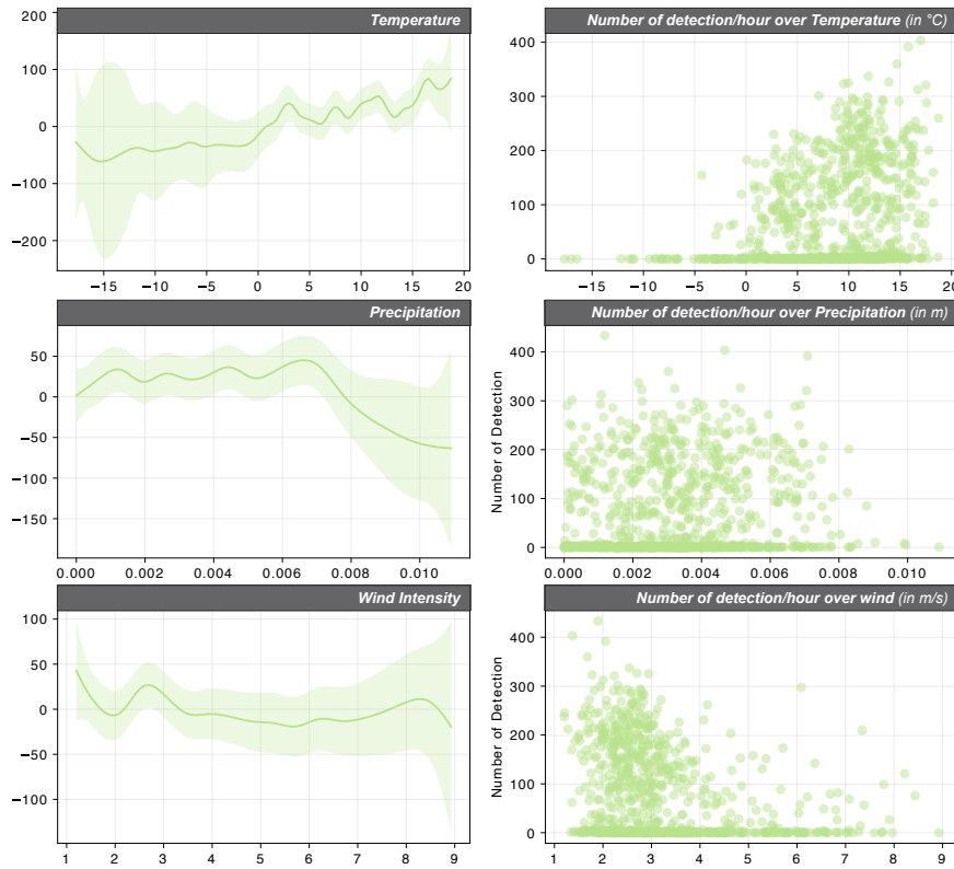
Figure 71: Results of the bird GAM with the response curves of temperature, total precipitation and wind intensity.
