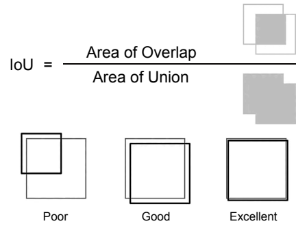
Figure 12: Representation of how the Intersection over Union (IoU) is measured and is evaluated
