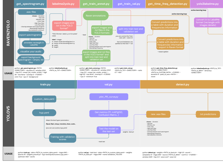
Figure 14: Workflow of the RAVEN2YOLO method
