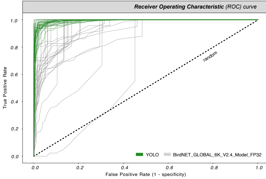
Figure 31: Receiver Operating Characteristic (ROC) curve of the 27 species for our model compared to BirdNET on the soundscape dataset from Québec, Canada database. The random classification is placed in dotted line.
