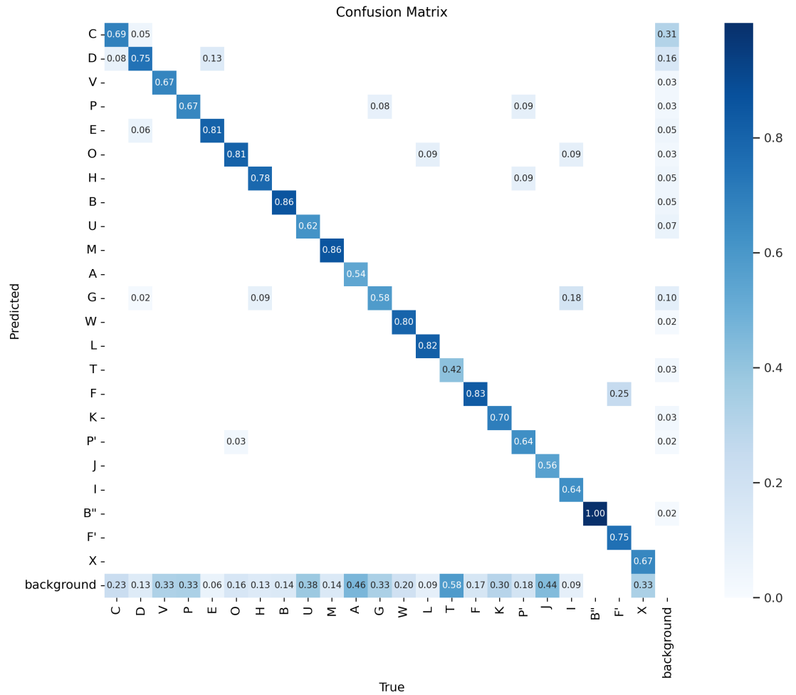
Figure 23: Confusion matrix of YOLO model over humpback whale units.
