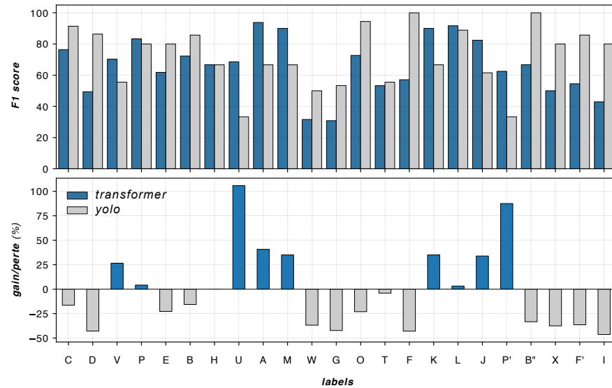
Figure 29: F1 score for the YOLO model compared to a transformer. The top part shows the F1 score for each model per unit type, while the bottom part shows the transformer's gain.
