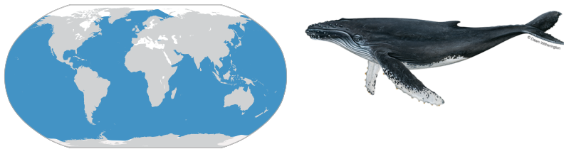
Figure 1: Humpback whale Distribution Map across the world. Map and illustration from : fisheries.noaa.gov
