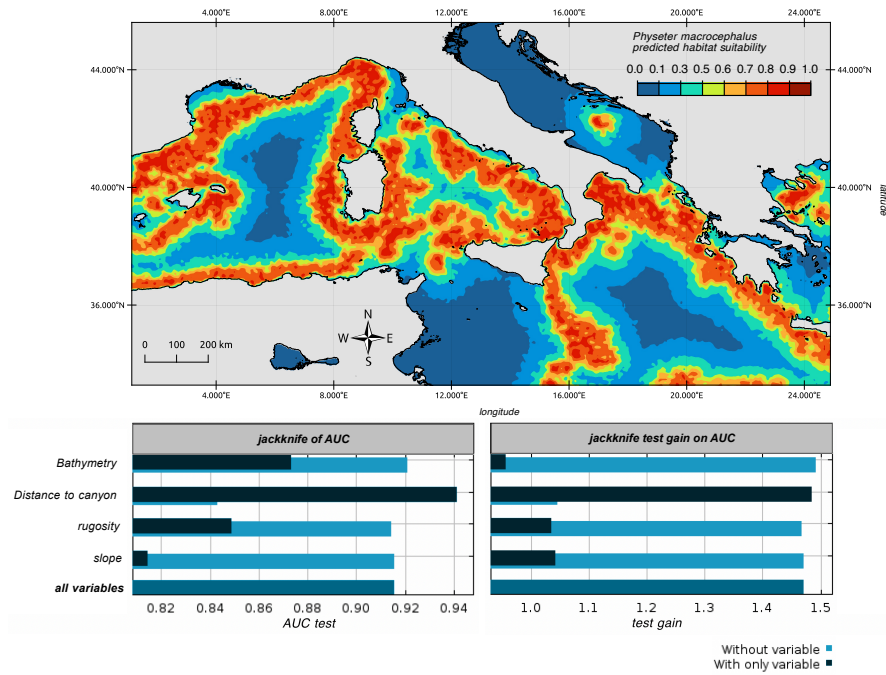
Figure 50: MaxENT model projection using all four fixed parameters, with the jackknife representation of the AUC and gain of each parameters.
