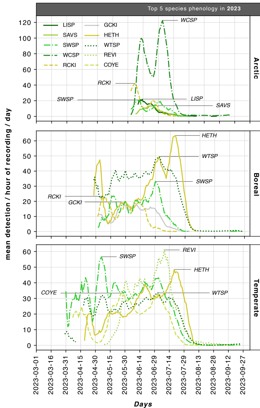
Figure 70: Mean detection per hour of recording for the 3 different areas for the top 5 detected species in 2023. The Arctic area, which is the one more at north have SWSP, WCSP, LISP, RCKI and SAVS as top 5 species while Boreal area has HETH, RCKI, GCKI, SWSP and WTSP. Finally, Temperate region, which is the more at south, has REVI, SWSP, COYE, HETH and WTSP as top 5 species.
