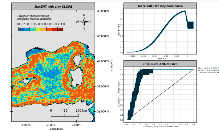
Figure 49: MaxENT model projection using the slope, with the response curve and its ROC AUC over the test set OBIS.
