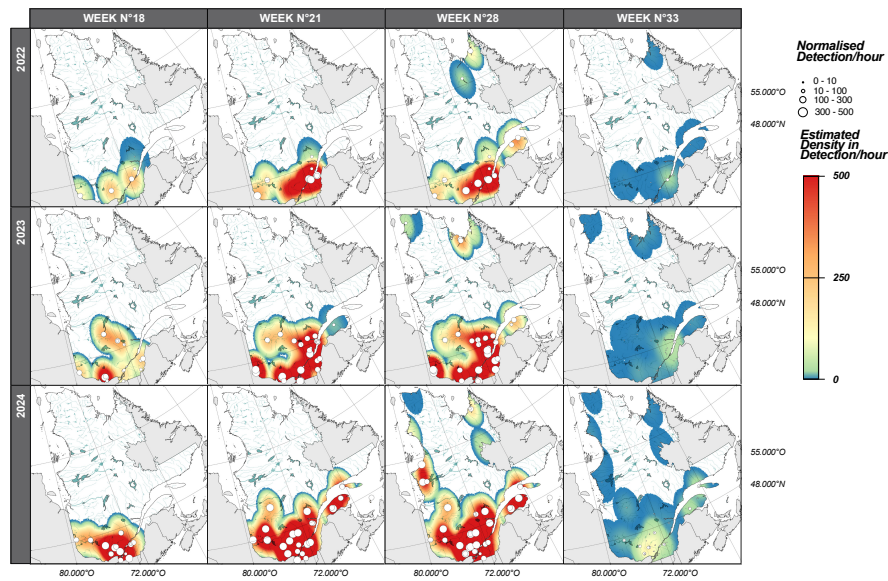
Figure 42: Evolution of detection density per hour of recording across Quebec between weeks 18 and 33 of 2022, 2023 and 2024.
