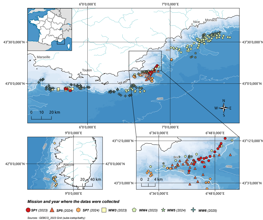
Figure 6: Map of the sperm whale observations from the different Longitude 181 missions in the Mediterranean Sea
