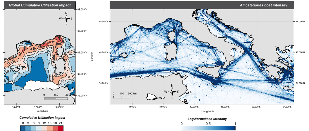
Figure 68: Result of the Cumulative Utilisation Impact of all boat categories summed together.
