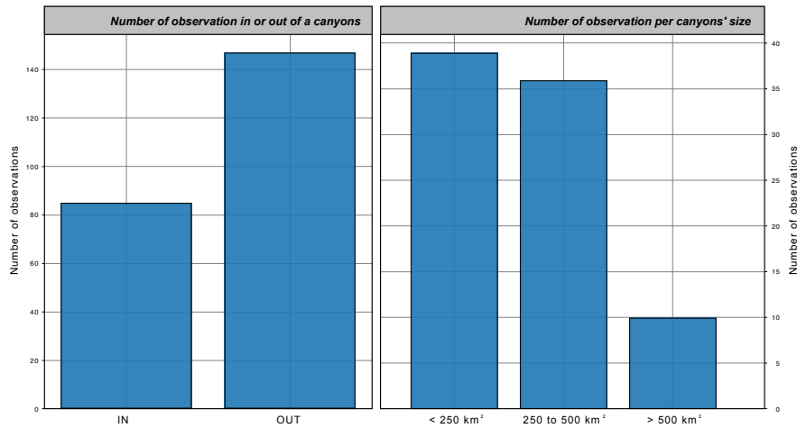
Figure 44: Number of sperm whale observations inside a canyon (with a 1.5km range around) compared outside (left) and the details of the canyon' surfaces (right)
