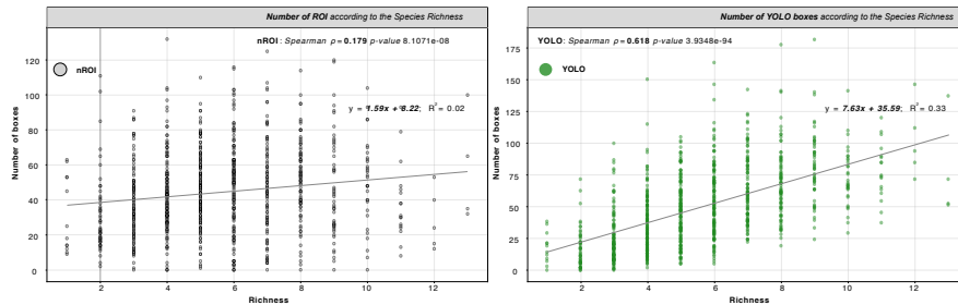
Figure 34: Number of detected boxes with the nROI index compared to the number of boxes from YOLO on the soundscape dataset from Québec, Canada database. The species richness take all the species in the recording, not only the one that compose the dataset.
