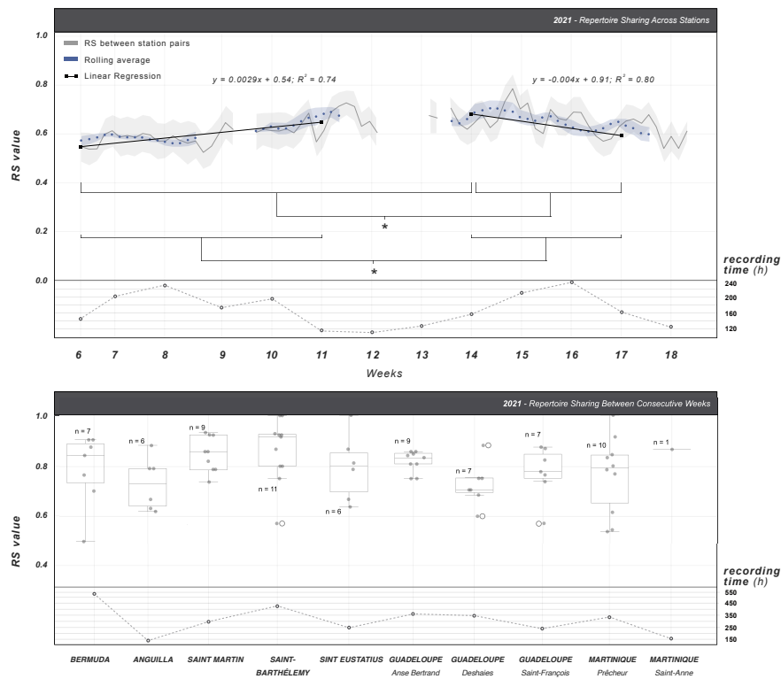
Figure 54: Spatial repertoire sharing as a function of time (top), and temporal repertoire sharing for each station (bottom). The top panel shows, per recording day, the RS between station pairs (with a standardised sampling effort). Temporal slopes of the spatial RS curve (in blue) are significantly different between the start and the end of the season. The bottom panel shows, per station, RS distributions for consecutive recording weeks, with boxes denoting Q1, Q2 and Q3 quartiles. *: p -value < 0.05
