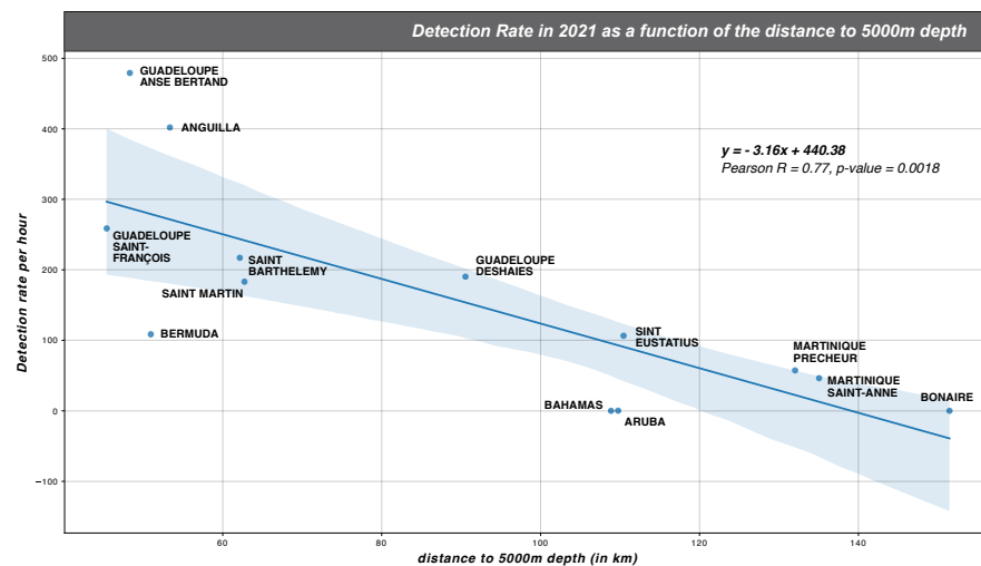
Figure 38: Detection Rate of humpback whale unit in 2021 as a function of the distance to 5000m depth.
