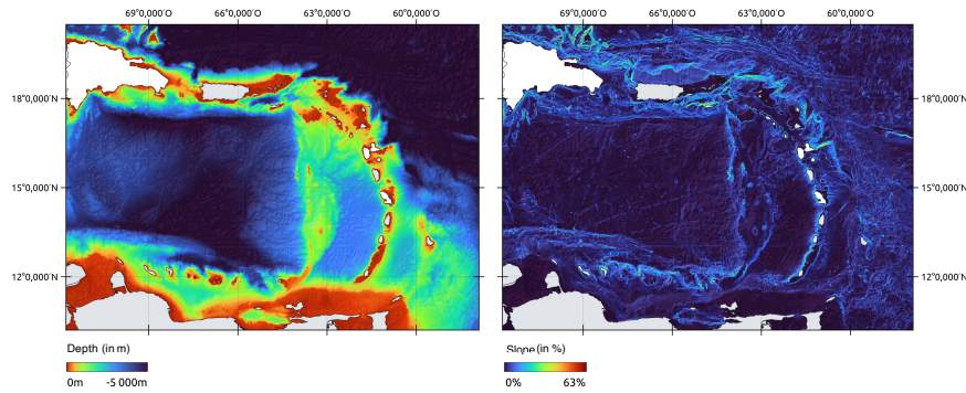
Figure 37: Bathymetric and slope map of the Caribbean region. The informations were extracted from the GEBCO 2023 dataset.
