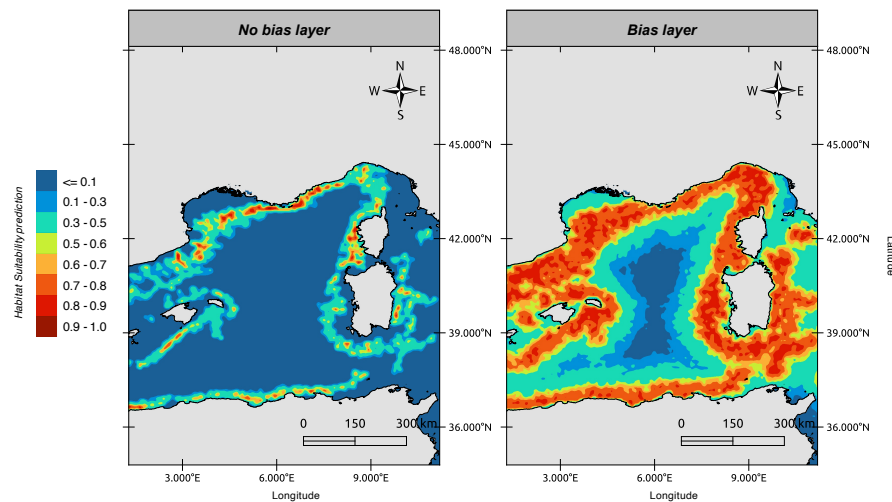
Figure 52: Comparison between a MaxENT model without bias layer (left) and with (right) using only fixed parameters.
