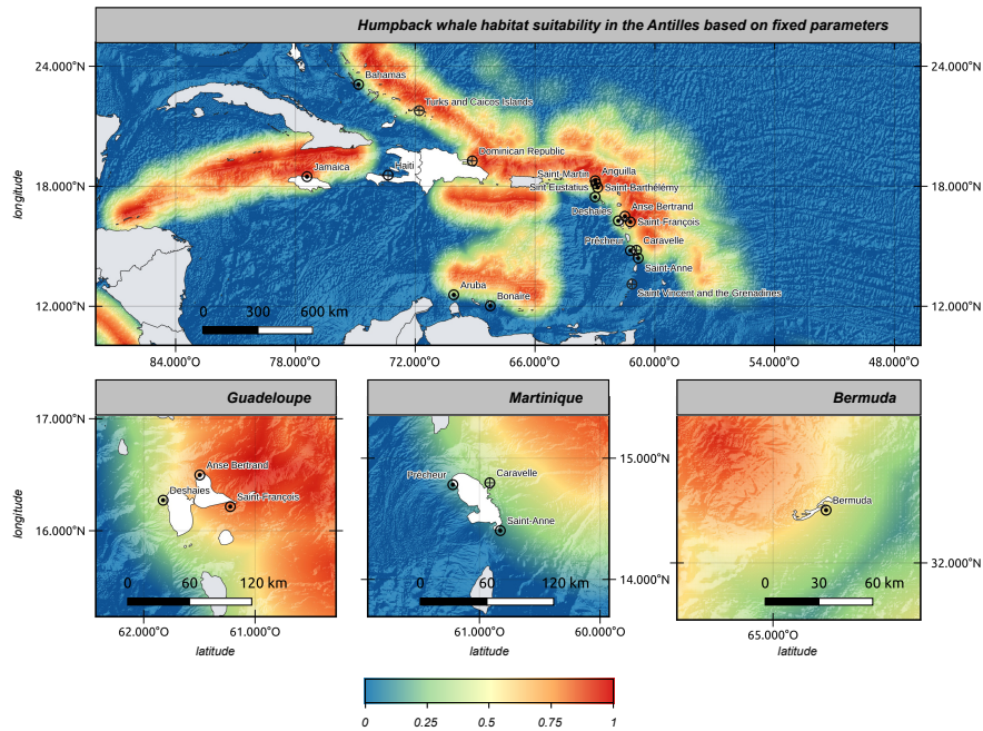
Figure 39: Predicted habitat suitability using the combination of the distance to the 5000 meter depth and the distance to the shore.
