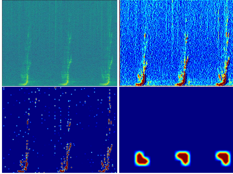
Figure 24: Original spectrogram (a) with the attention map extracted from the model, at the layer 0 (b), layer 1 (c) and -2 (d)
