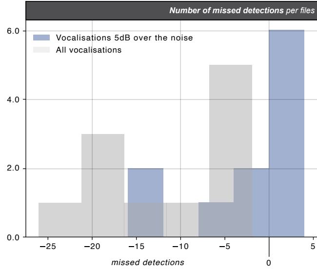
Figure 26: Post hoc analysis of the missed detection per file over 11 files. The y-axis corresponds to the number of files for which x units were missed, while the x-axis is the number of units missed.
