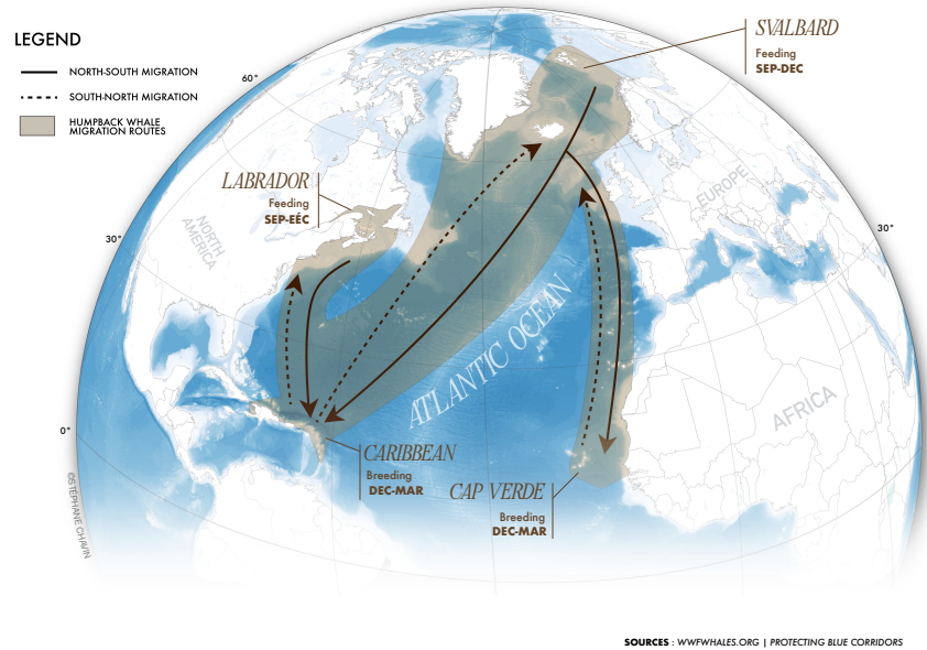
Figure 2: Megaptera novaeangliae North Atlantic Population Migration Map
