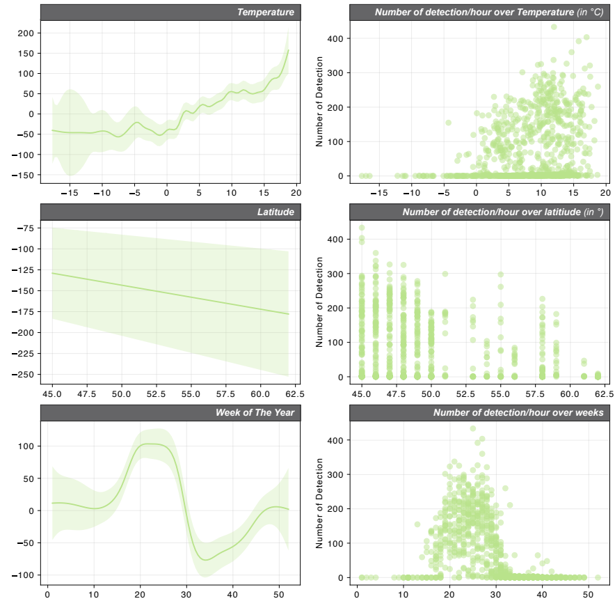
Figure 72: Results of the bird GAM with the response curves of temperature, latitude and week number.
