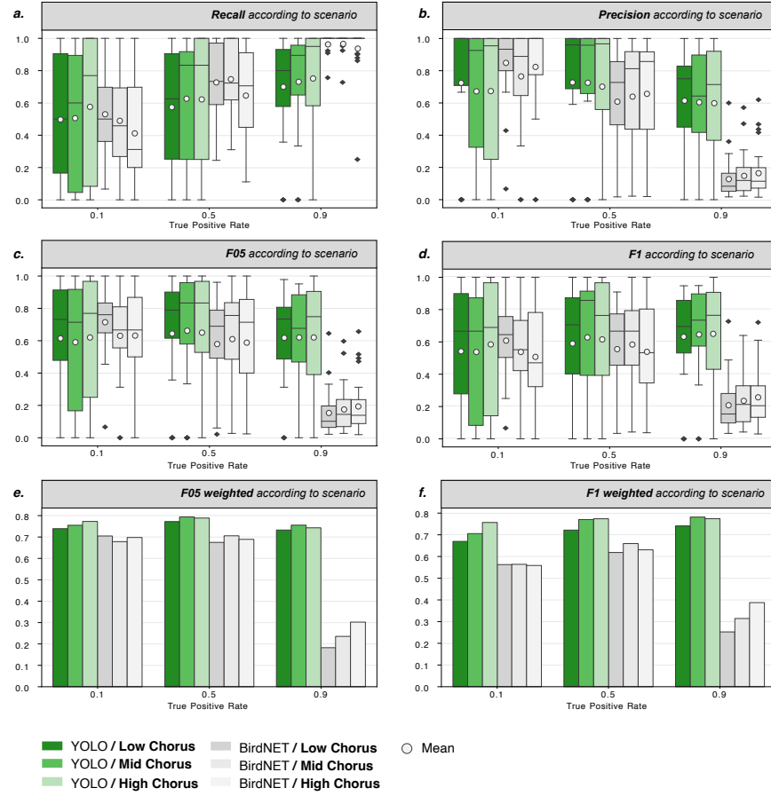
Figure 32: Evaluation of our model and BirdNET over the three different scenarios on the soundscape final validation dataset. The average for each metric is represented by a dot.
