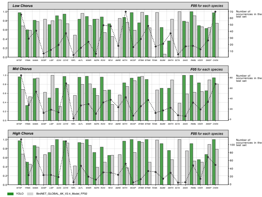
Figure 33: F0.5-score for BirdNET at a true positive rate scenario of 0.1 and our model at a true positive rate scenario of 0.5 for the 27 species on the soundscape dataset from Québec, Canada database. The dotted line represent the number of each species to detect in each chorus level.
