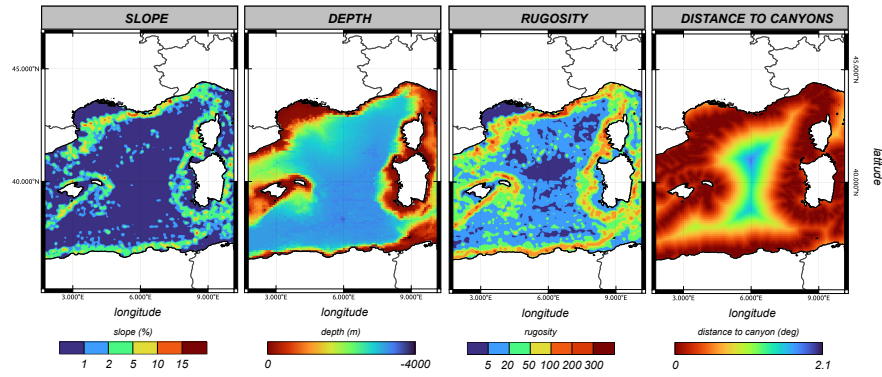
Figure 45: Fixed parameter maps with slope (a) depth (b) rugosity (c) and distance to canyons (d) in the western basin of the Mediterranean
