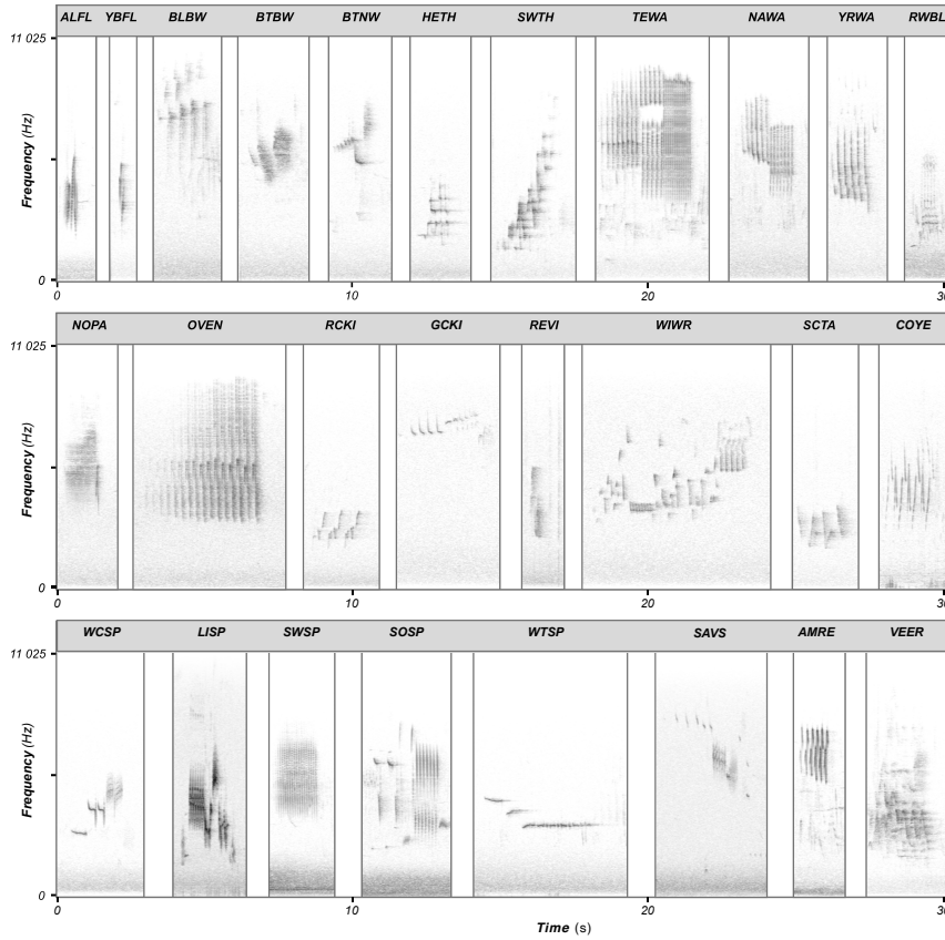
Figure 19: 27 bird species repertoire. All spectrograms were generated using a Short-Term Fourier Transform (STFT) (signals sampled at 22,050 Hz, 300 Hz High Pass filter, 9000 Hz Low Pass filter, 2048-point Hanning window and 90% overlap)
