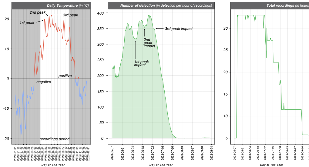
Figure 83: Daily temperature and detection rate with total recording time for 2023 season in the Abitibi Témiscamingue region.
