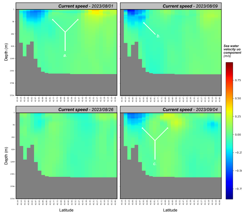
Figure 79: Current eastward component evolution during different days for a depth latitudinal cut. a. their is the Northern current and the Balearic one; b. the Northern current is closer to the shore, and stronger, it can create downwelling; c. the Northern current and Balearic front is again and closer, with the increase of current in the deep
