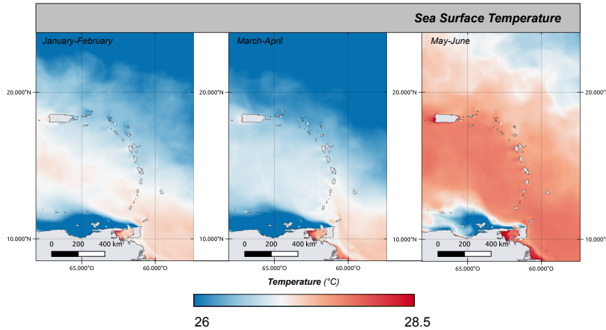
Figure 60: Temperatures over 3 periods of time in the Caribbean.
