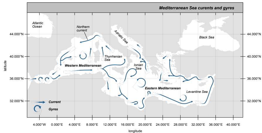
Figure 53: Mediterranean Sea global current. This map, adapted from [155], shows the different currents and gyres inside the Mediterranean Sea's various regions.
