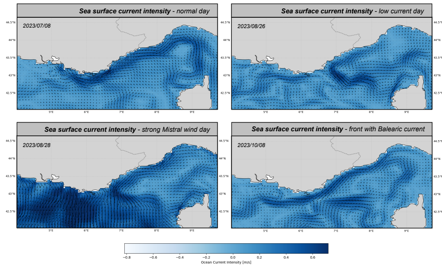
Figure 77: Different sea surface current conditions with different event types.
