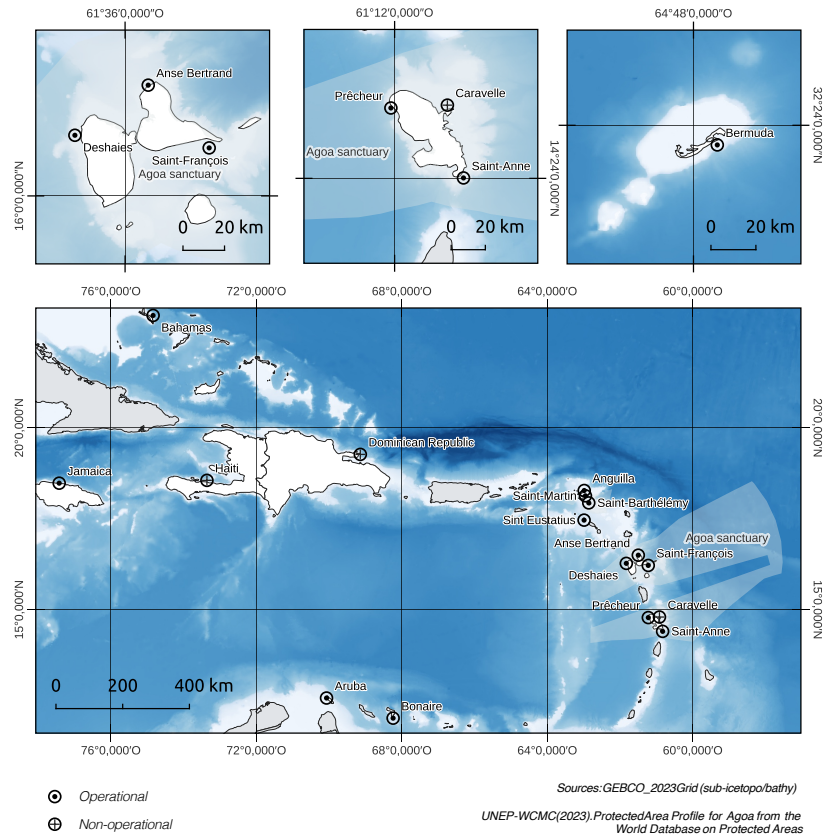
Figure 5: Map of the different ARU positions in the Caribbean region, from Bermuda to Aruba
