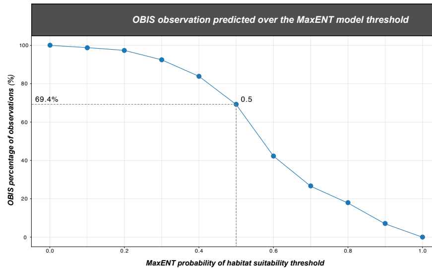
Figure 66: Proportion of OBIS observation predicted inside area depending on our model confidence.
