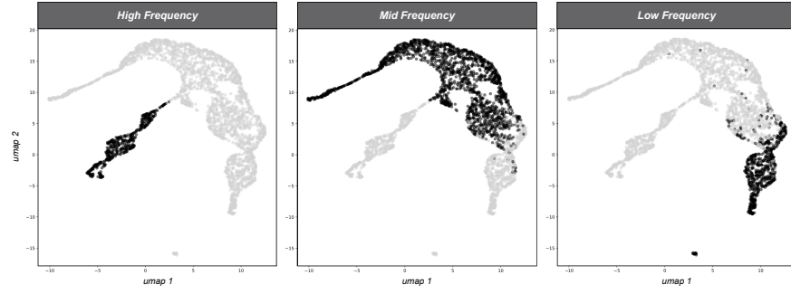
Figure 16: Representation of the humpback whale vocal repertoire categories using 2 dimension UMAP
