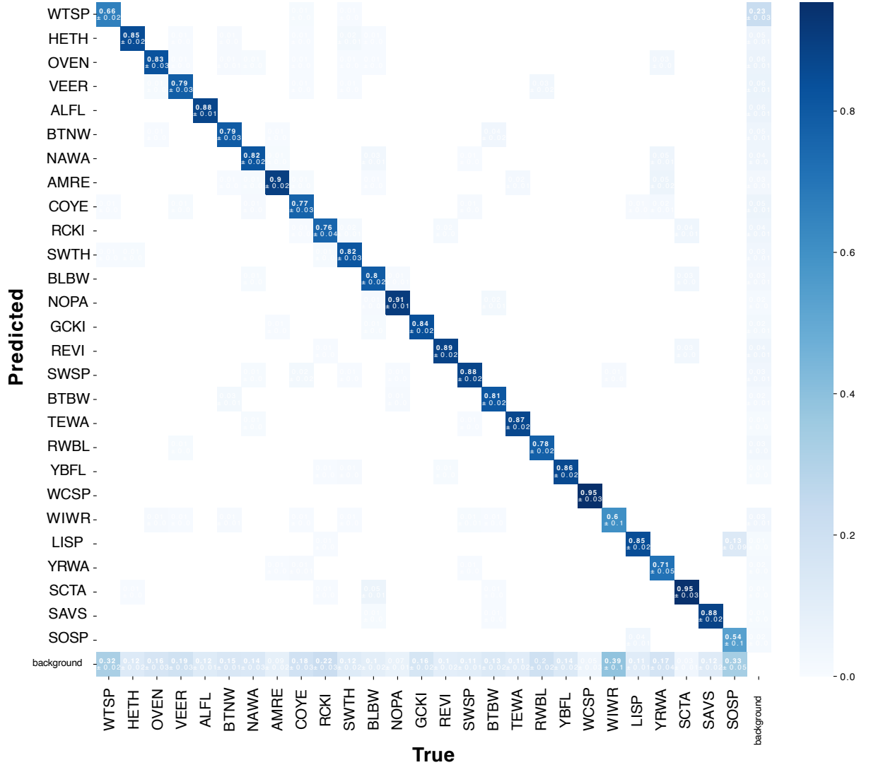
Figure 30: Confusion matrix on the test set of the annotations from the Québec, Canada database, with a total of 27 species. The standard deviation is measured with the Kfold cross validation with k = 10 . The X-axis corresponds to the annotations, while the Y-axis shows the model's predictions. Diagonals indicate good predictions, while background predictions correspond to missed annotations.
