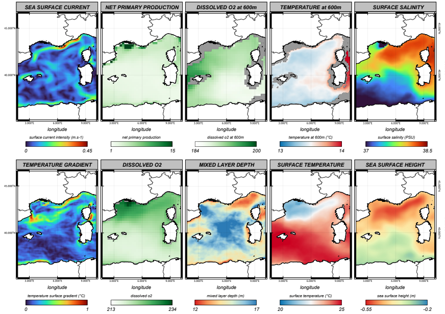
Figure 63: Mediterranean dynamic parameters averaged between May and October.
