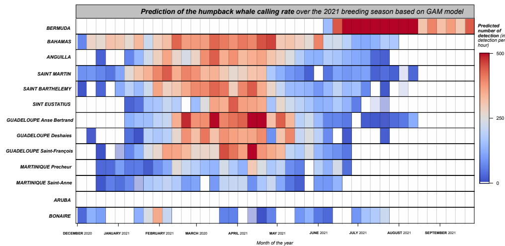
Figure 62: GAM prediction of the rate of humpback whale calls over the entire breeding ground throughout the 2021 breeding season and until the end of September.
