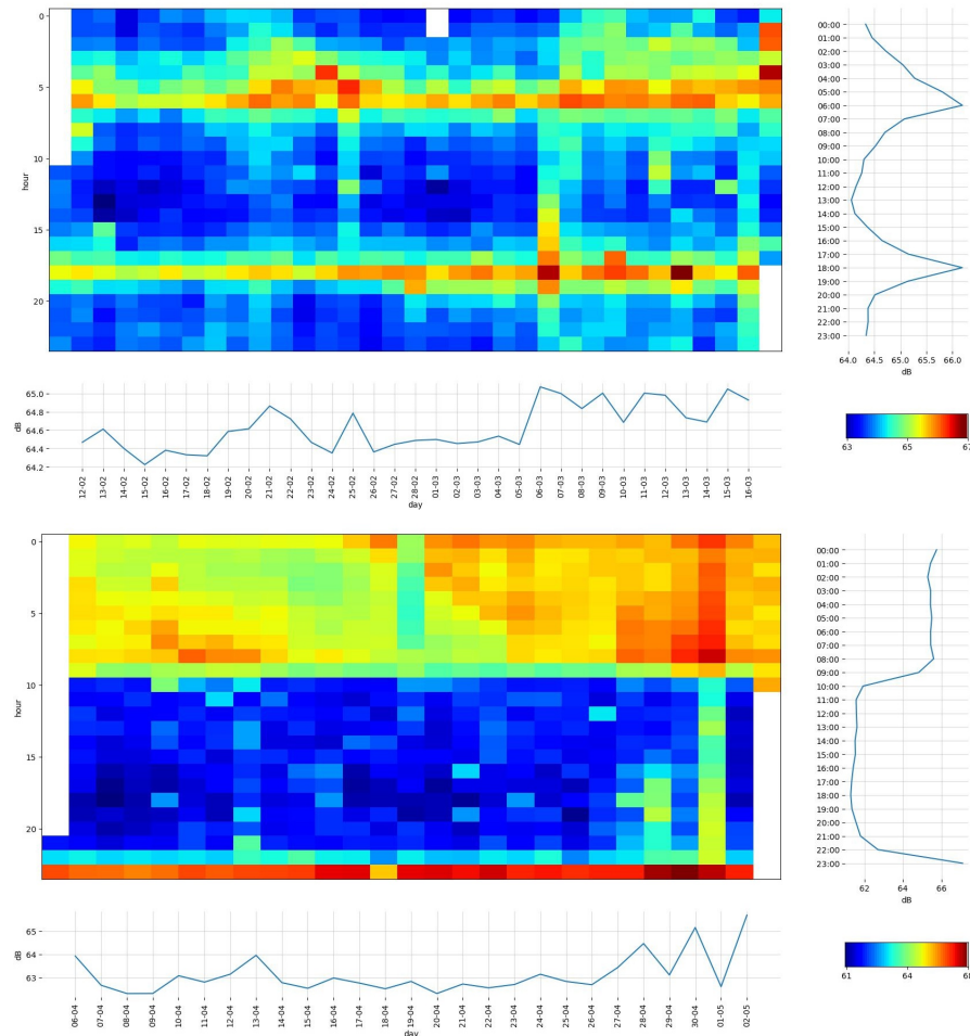
Figure 84: Evolution of the decibel levels for a. Guadeloupe Anse Bertrand and b. Guadeloupe Deshaies between 6500 and 12500Hz
