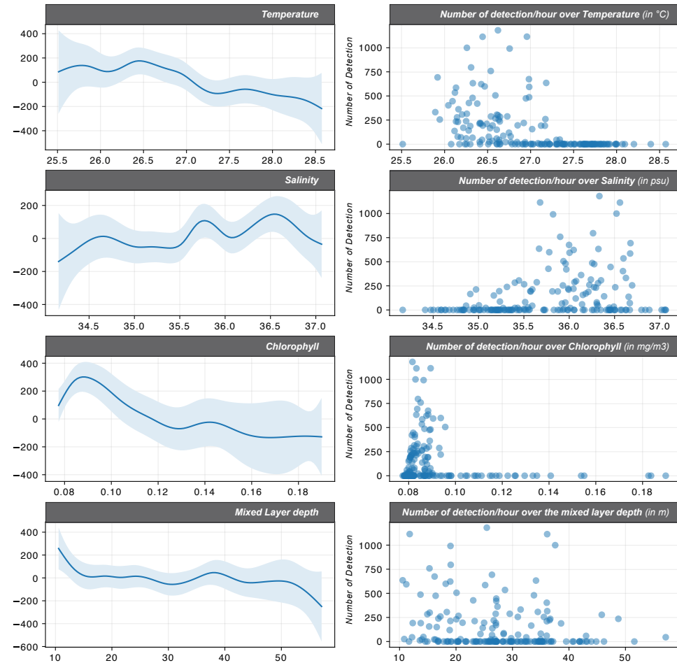
Figure 56: Results of the humpback whale GAM with the response curves of its components.
