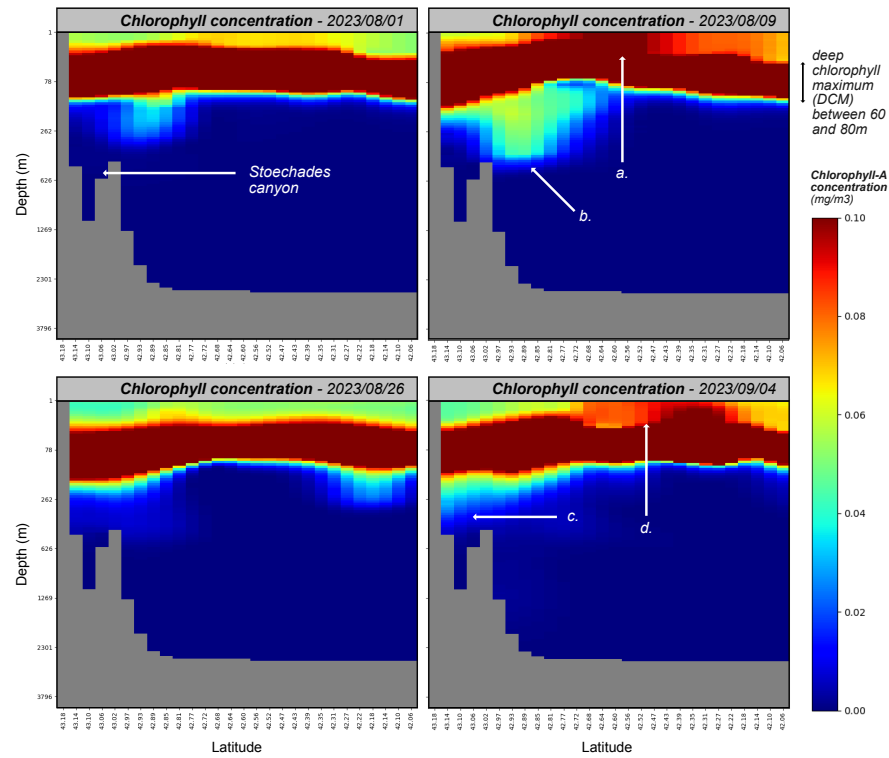
Figure 78: Chlorophyll concentration during different days for a depth latitudinal cut. a. the surface chlorophyll concentration is high; b. There is a big increase of the concentration of chlorophyll-a in the deep (up to 600m); c the deep chlorophyll is high into the canyon; d : the surface chlorophyll increase again in the surface.
