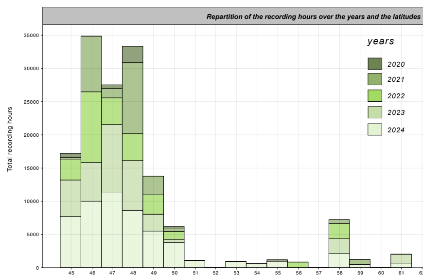
Figure 40: Distribution of the total recording time in hours for each year, depending on the latitude of the station
