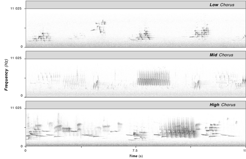
Figure 20: Representation of the different levels of Chorus in the dataset. Top panel represents a low chorus, without overlap, the middle panel shows a mid chorus, with little overlap while the bottom panel represents a high chorus with much overlap.
