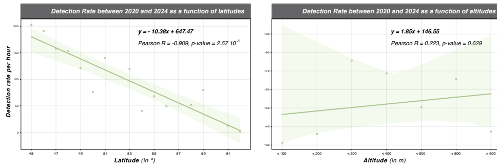
Figure 41: Linear regression between the detection rate and the latitudes (a.) and altitudes (b.).
