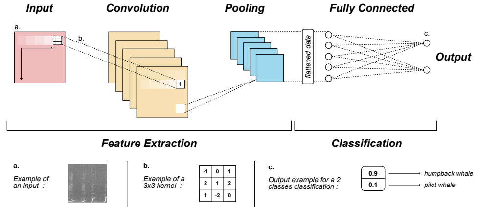
Figure 11: Main part of a convolutional neural network, with the example of a humpback whale song spectrogram.
