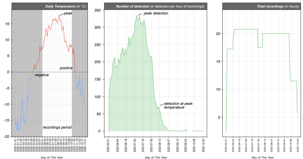
Figure 82: Daily temperature and detection rate with total recording time for 2022 season in the Côte-Nord regions.
