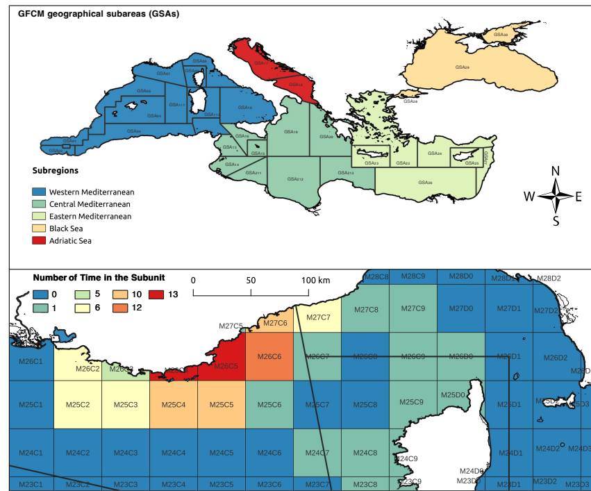
Figure 7: Geographical sub areas and subunits with the sampled area during Longitude 181 missions
