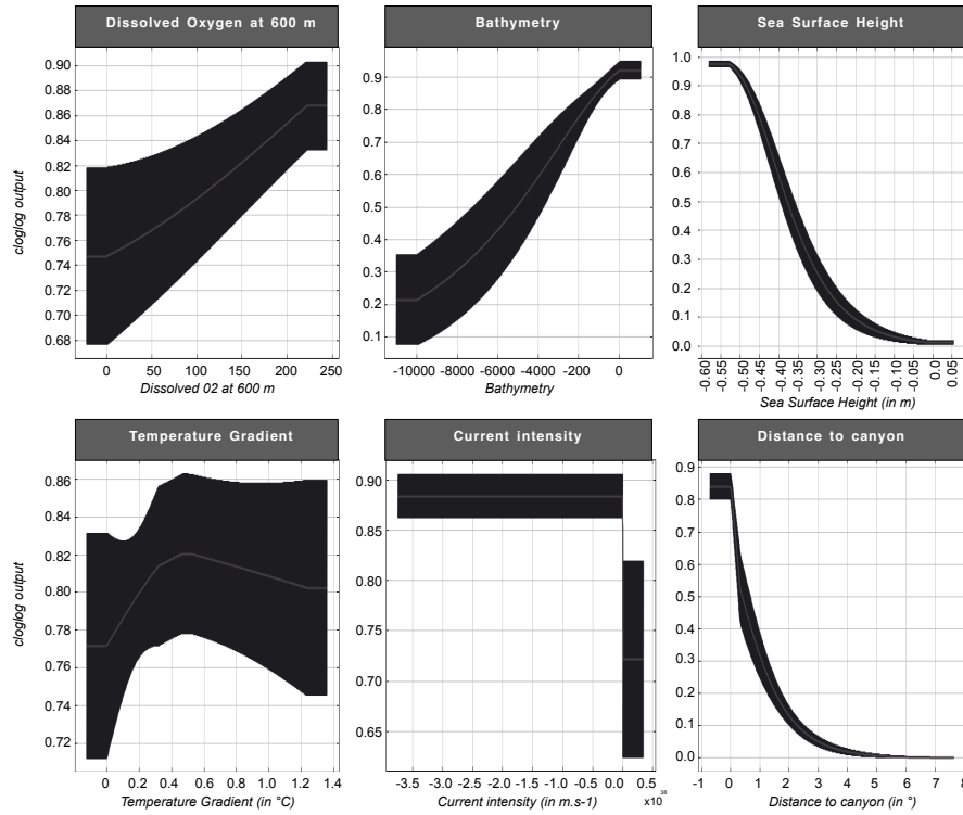
Figure 65: Response curve of some of the parameters that composes the MaxENT model.
