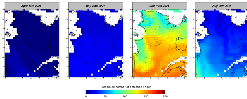
Figure 73: Prediction of the potential birds distribution across Québec at different times of 2021 based on the GAM.
