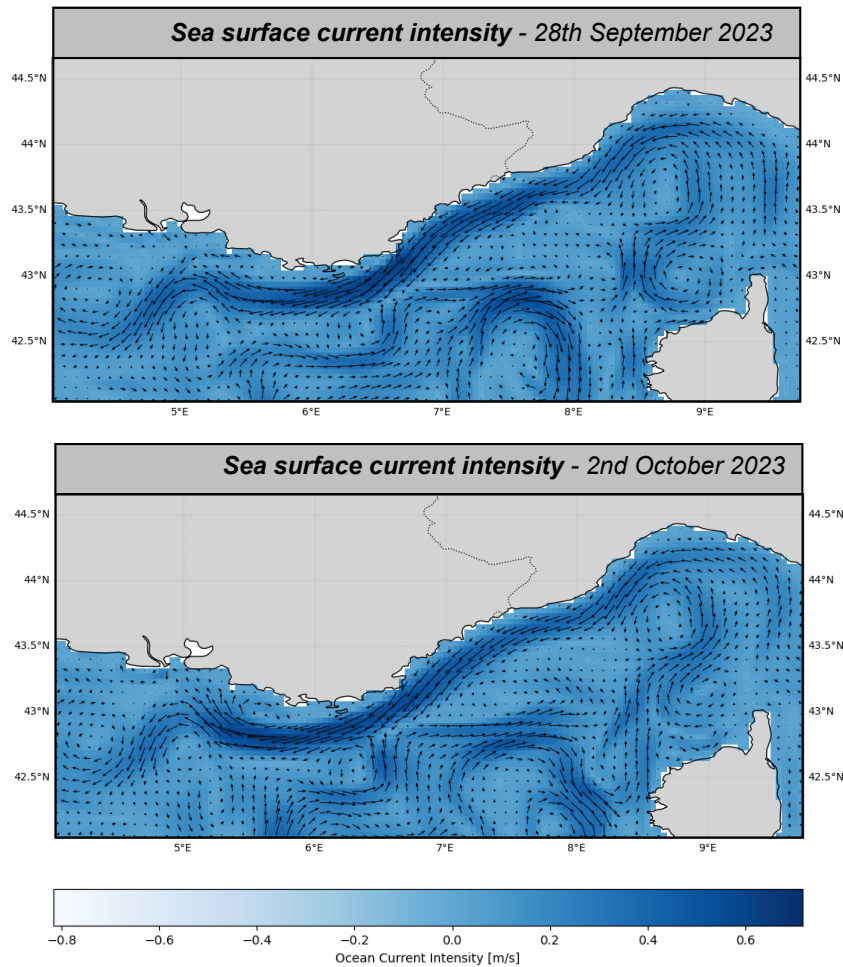
Figure 81: Sea surface current orientation on the 28th of September and 2nd of October with a front off-shore the islands of Hyères.
